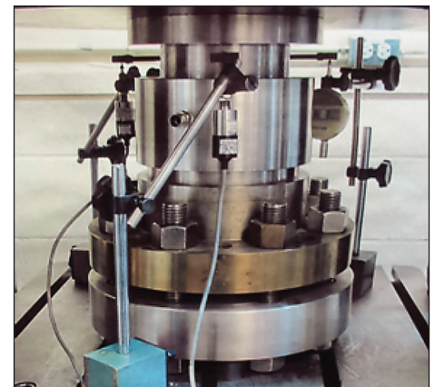
Fixture testing.
