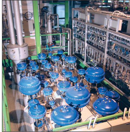
Some of the 2,500 Velan cryogenic valves for liquid helium installed in the Large Hadron Collider (LHC) at CERN.
