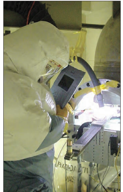
In-line seat removal and seat welding and lapping, performed in association with global field services.
