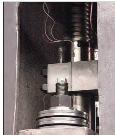
Velan delivers valves with pre-installed thrust and torque sensors, signal conditioners and cabling (smart stems).
