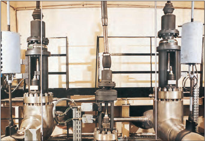
Velan valves in a cooperative program for qualification testing with Électricité de France at their R&D facility in Renardière.
