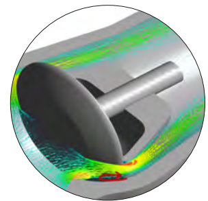
Minimize recirculation zones
