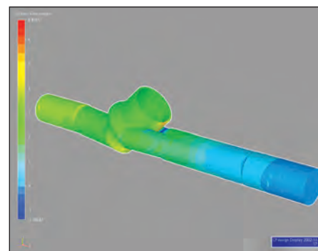
Velan used computational fluid dynamics to improve the flow characteristics of this NPS 4 (DN 100) globe valve.
