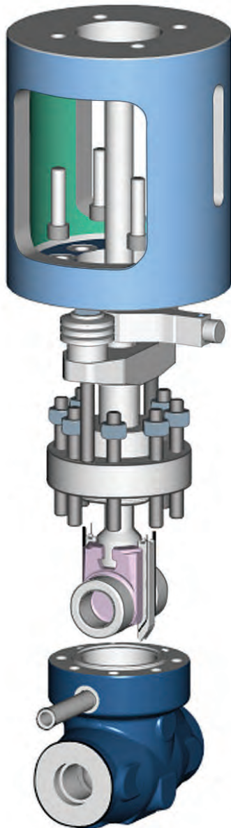
Next generation gate valves developed by Velan to meet the requirements of major North American utilities.
