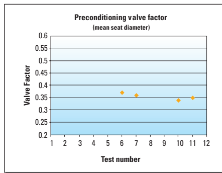
Two graphs from the Wyle test report results show the preconditioning stem factor and valve factors based on the mean seat diameter.
